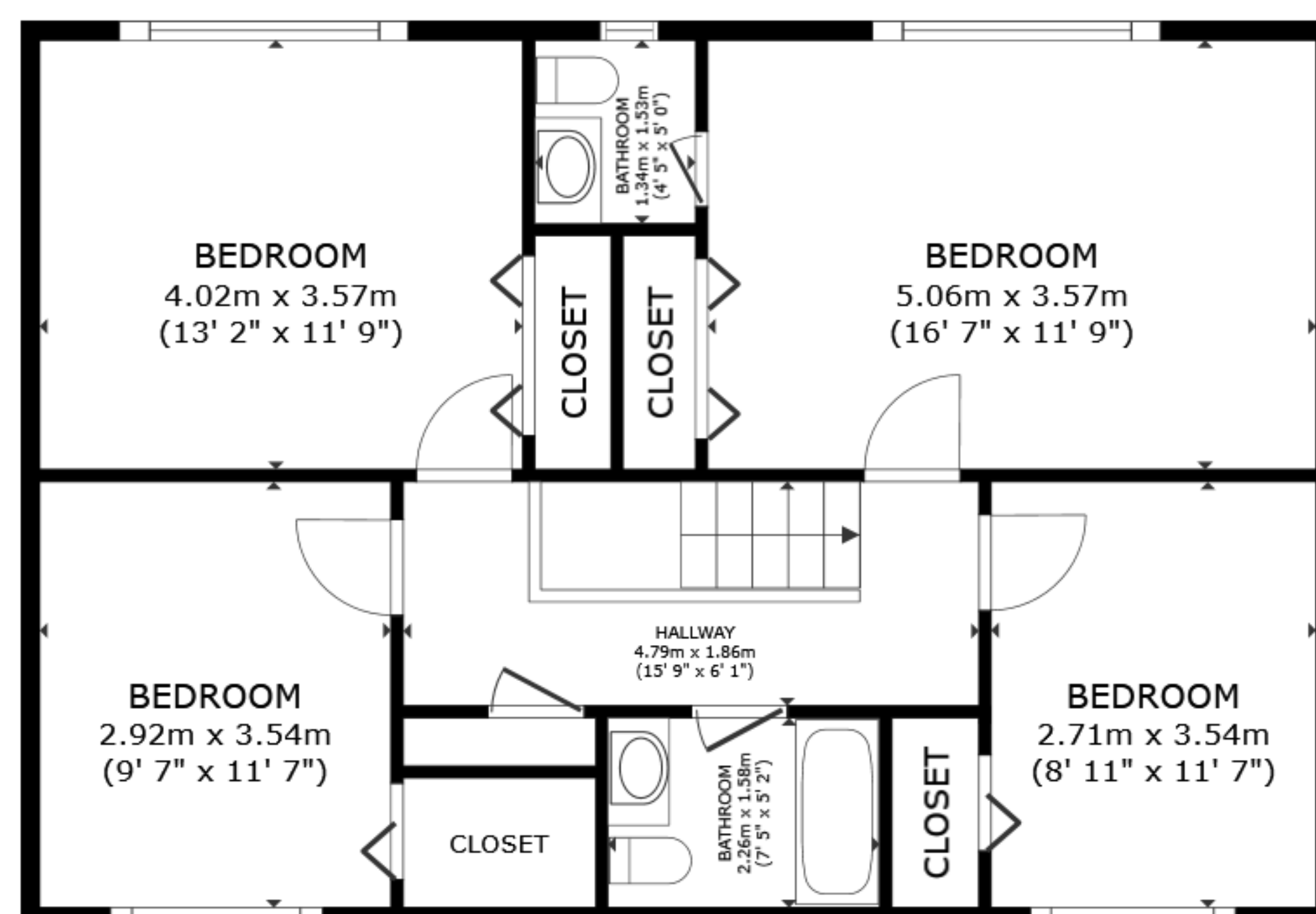
FLOOR 2
